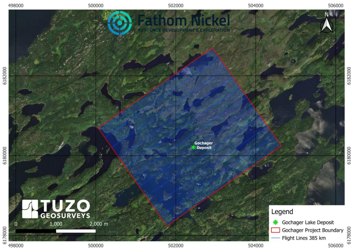
Figure 3 – Tuzo Geosurveys Drone-MAG Survey Area
