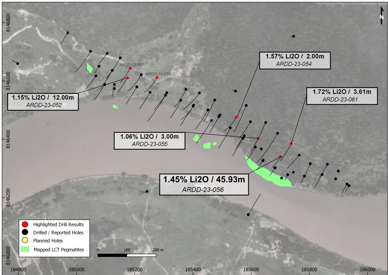
Figure 2: Galvani Plan Map with Latest Drill Results
