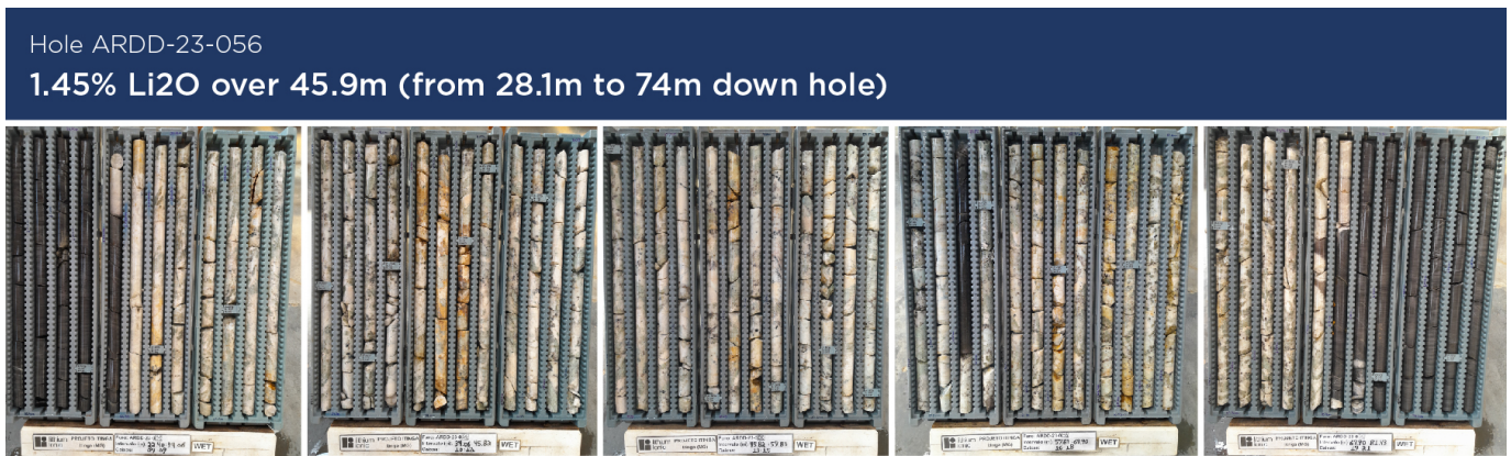
Figure 3: Core photo of holes ARDD-23-056
