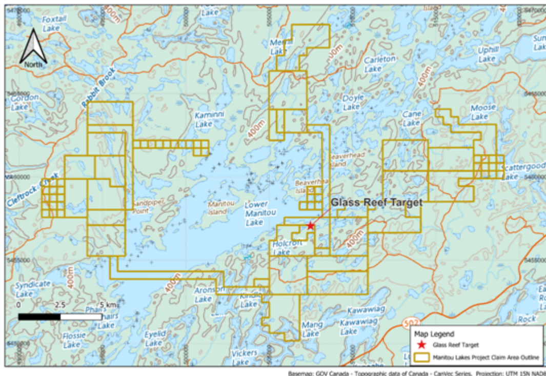
Figure 1: Location of the Glass Reef Target within the Manitou Lakes Project
