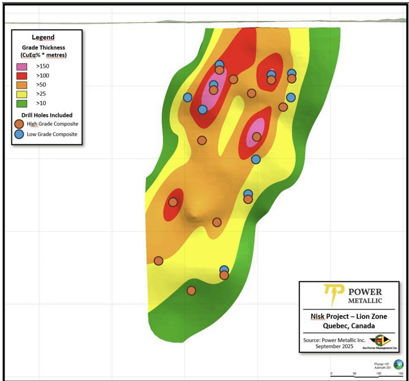
Figure 1 Spatial distribution of the drill hole intercepts used in the Metallurgical Testing (CNW Group/Power Metallic Mines Inc.)
