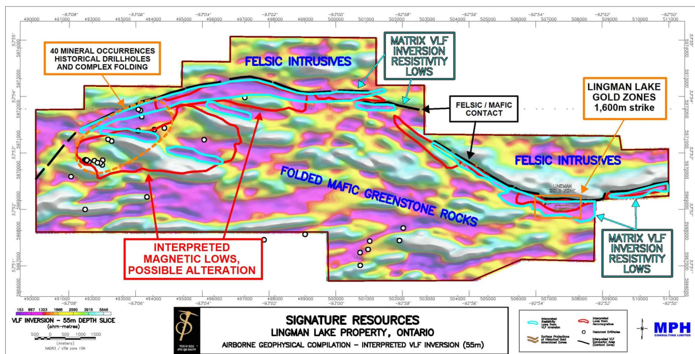
Figure 2 – An image of the VLF-EM 55-meter depth inversion slice from the airborne survey is presented below. The resistivity lows from the VLF inversion are correlated with the magnetic lows, mentioned above in Figure 1. Combined, these may indicate prospective target zones along the felsic/mafic contact.
