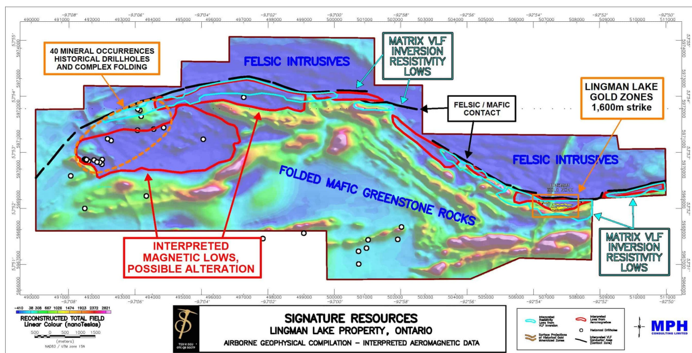
Figure 1 – An image of the Reconstructed Total Field magnetics from the airborne survey is presented below highlighting key areas. The felsic intrusives are obvious magnetic lows, but this presentation shows distinct magnetic lows immediately South of the felsic/mafic contact, which could relate to alteration and magnetite replacement by pyrite.
