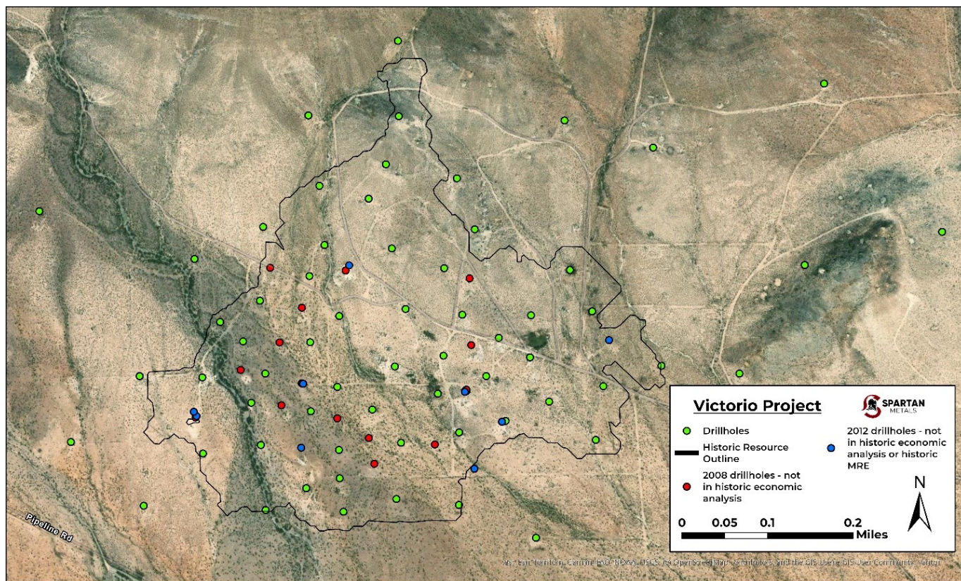
Figure 2: Plan view drill hole map of Victorio Tungsten-Molybdenum Project highlighting core holes not included in historic 2008 economic analysis and/or the historic 2012 Mineral Resource Estimate
