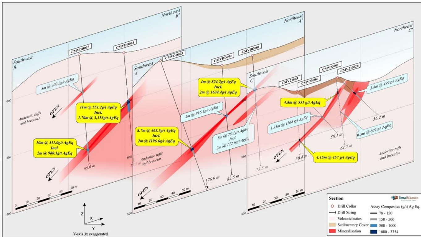
Figure 2. Fence diagram of Phase I and II drilling completed at the Cumavici Ridge target. Polymetallic mineralization intervals are highlighted in red. The mineralization remains untested and open down dip to the southwest and entirely open to the NW. The high-grade mineralization footprint currently sits at approximately 92 m (strike length) by 150 m in down dip direction ( click here to view image ).
