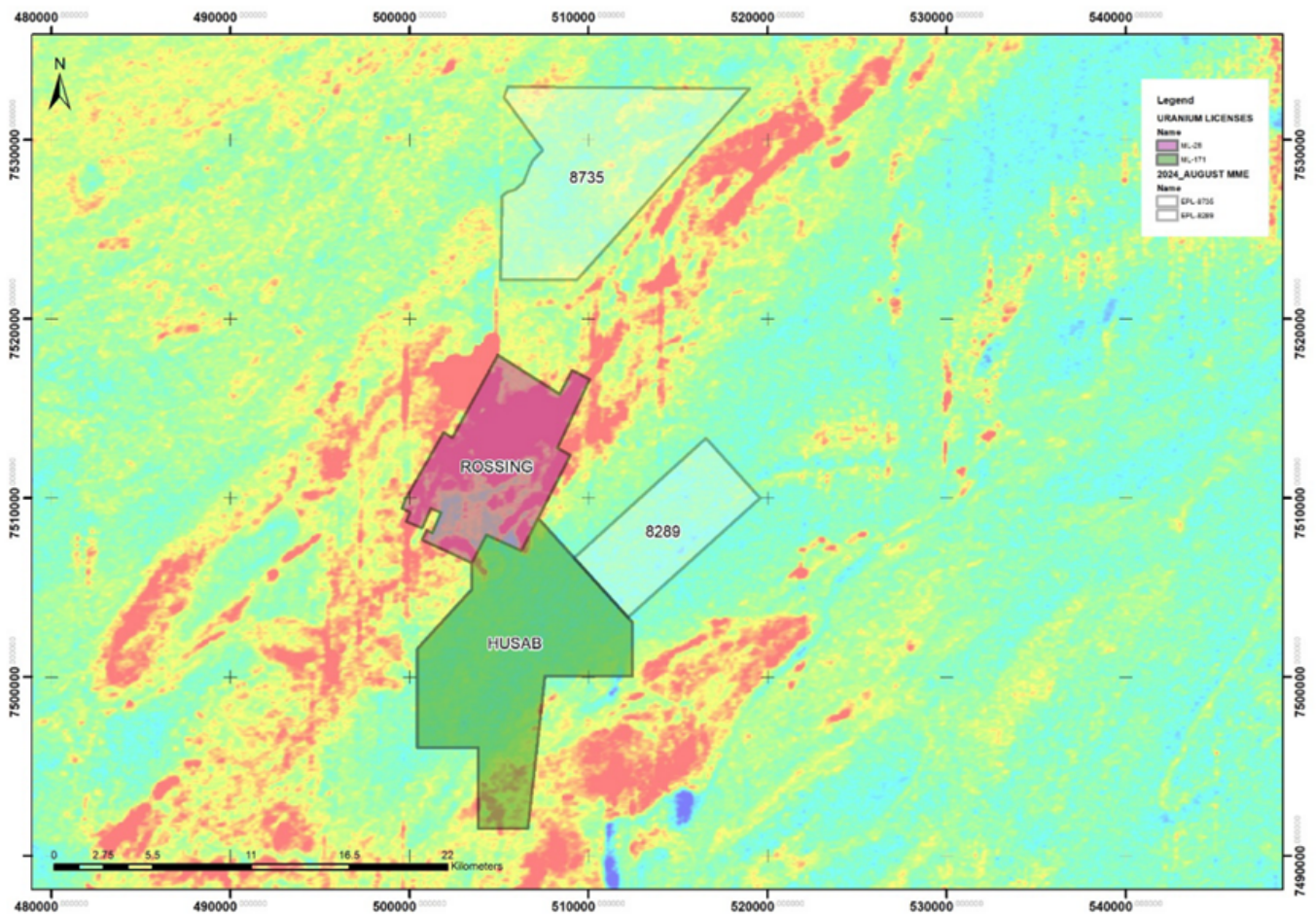
Figure 2: Map showing EPL 8289 and EPL 8735 within the Alaskite Alley on uranium channel airborne radiometric data (200 m line spacing and 80 m flight height) acquired from the Geological Survey of Namibia. Note the setting of the EPLs in vicinity to the Rossing and Husab uranium mines.
