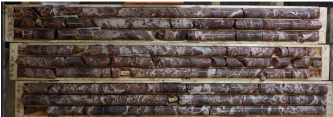
Figure 3. SL26-30 high-grade TREO and Ga mineralization in red syenite and white carbonatite, 130.5m – 144.1m, boxes 32–34.
