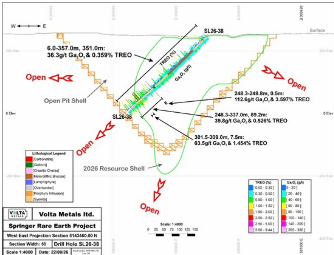
Figure 5. Cross section for drill hole SL26-38.
