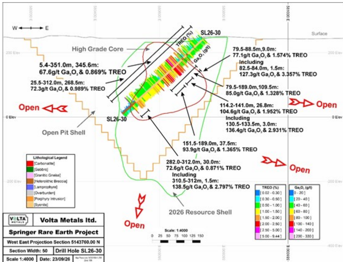
Figure 4. Cross section for drill hole SL26-30.
