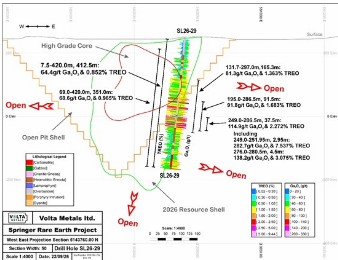
Figure 2. Cross section for drill hole SL26-29.
