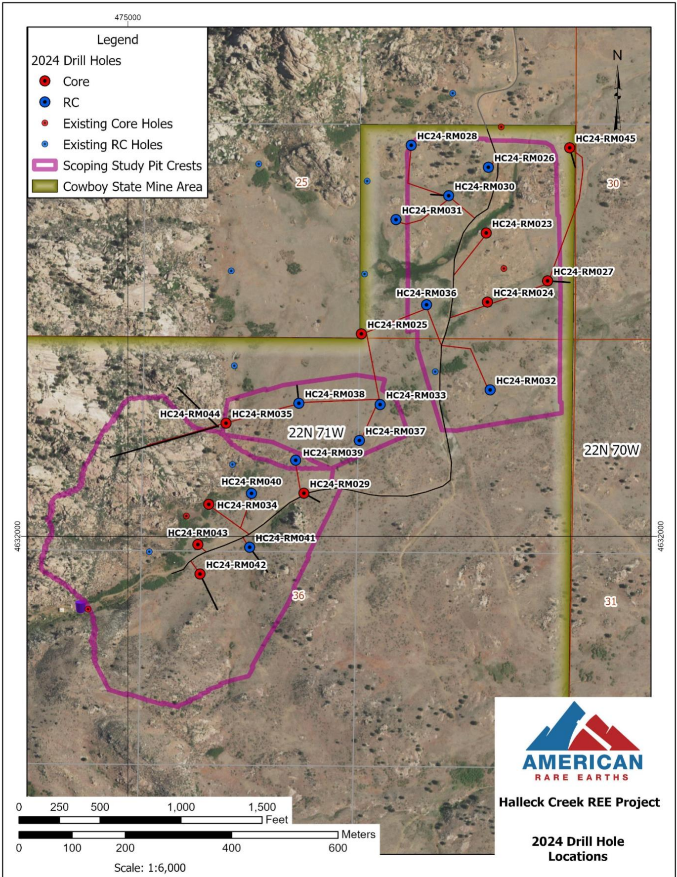
Figure 1 – 2024 Drill Hole Locations
